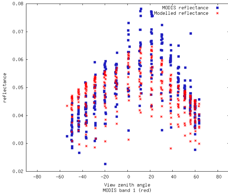
Band 1 (red)
