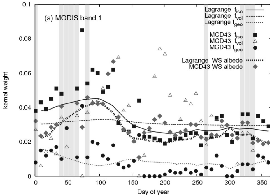
Band 1 (red)
