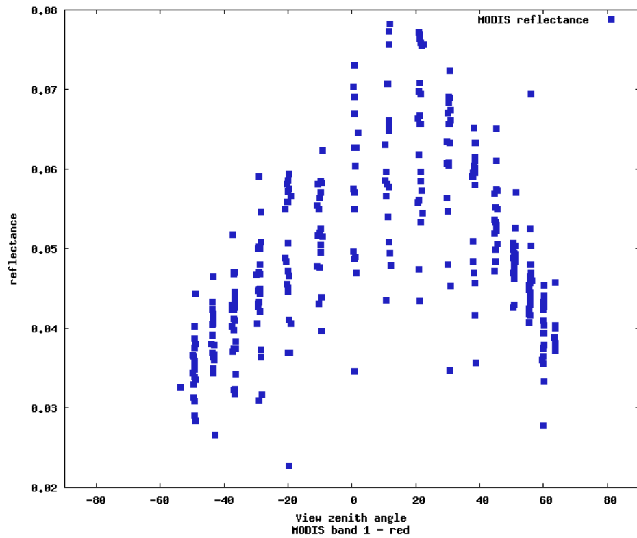
Band 1 (red)
